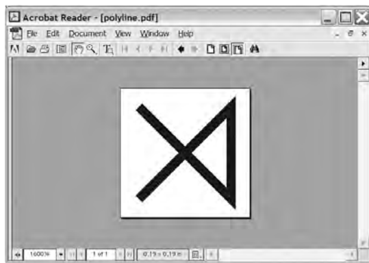
图21-2 PolyLine([(0, 0), (10, 0), (10, 10), (0, 10)])
